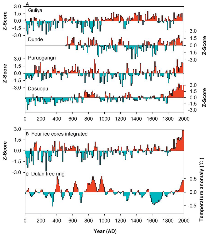
FIG. 1. Ice core and tree-ring climate records in the TP (red = warm climate; blue = cold climate). (a) 10-yr averages of \delta^{18}\text{O} in the past 2,000 years recorded in the Guliya, Dundee, Puruogangri, and Dasuopu ice cores. (b) Temperature change curve in the past 2,000 years in the TP reconstructed from the four ice cores. (c) Temperature change curve in the past 2,000 years in the TP reconstructed from tree rings. The z score in the figure refers to the normalized anomalies, which consider both mean and standard deviation
