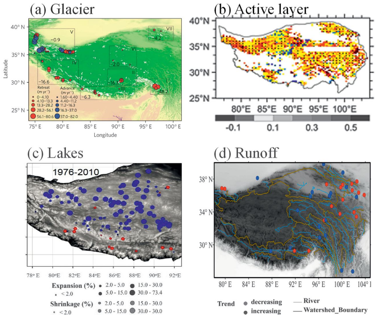
FIG. 3. (a) Observed changes in glacier (m yr -1 ; from Yao et al. 2012b), (b) simulated changes in active layer thickness during 1981–2010 (m decade -1 ; from Guo and Wang 2013), (c) observed changes in lake areas during 1976–2010 (from Lei et al. 2014), and (d) runoff change based on hydrological station data (modified from Cuo et al. 2014).
