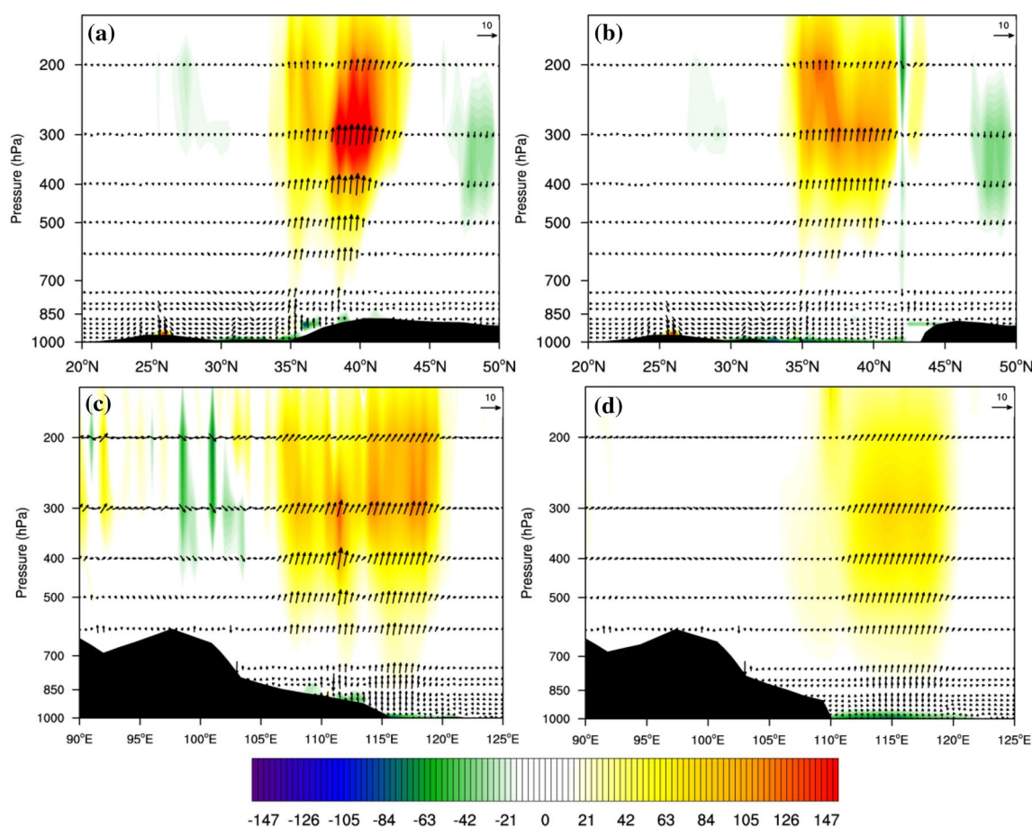
Fig. 10 The composite latitudinal and meridional cross sections of atmospheric apparent heat source Q_1 (contour; unit: 10^{-4} \text{ m}^2 \text{ s}^{-3} ) and wind fields for the six extreme precipitation days in the control test
